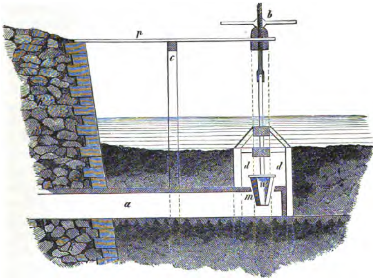
Fig. 240.—Plug-valve.
